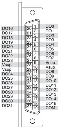
Figure 2. NI 9476E Pin Assignments
